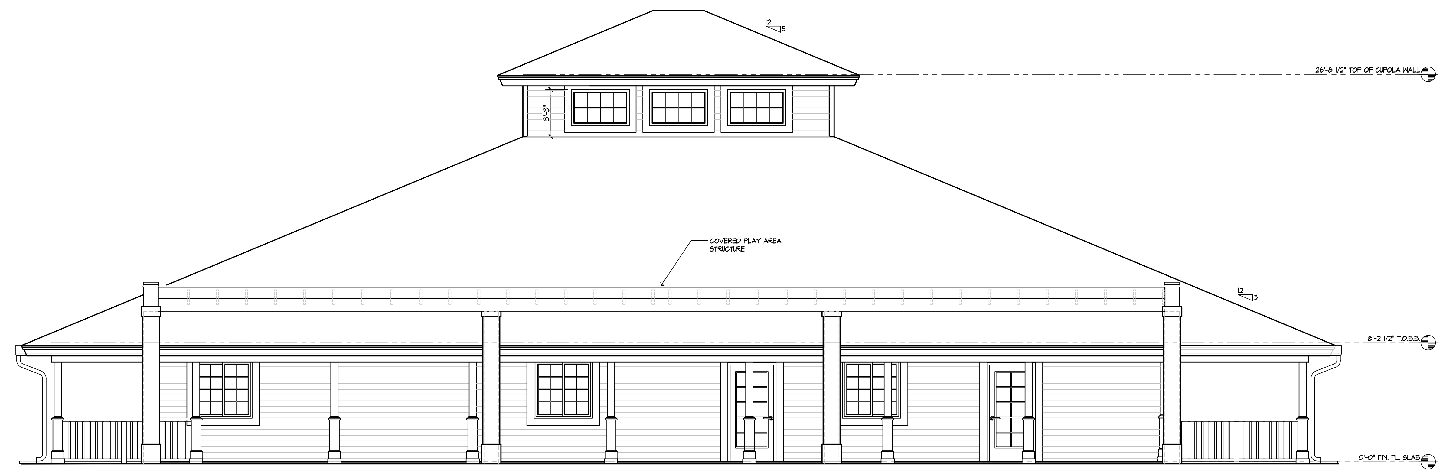
LEFT ELEVATION
