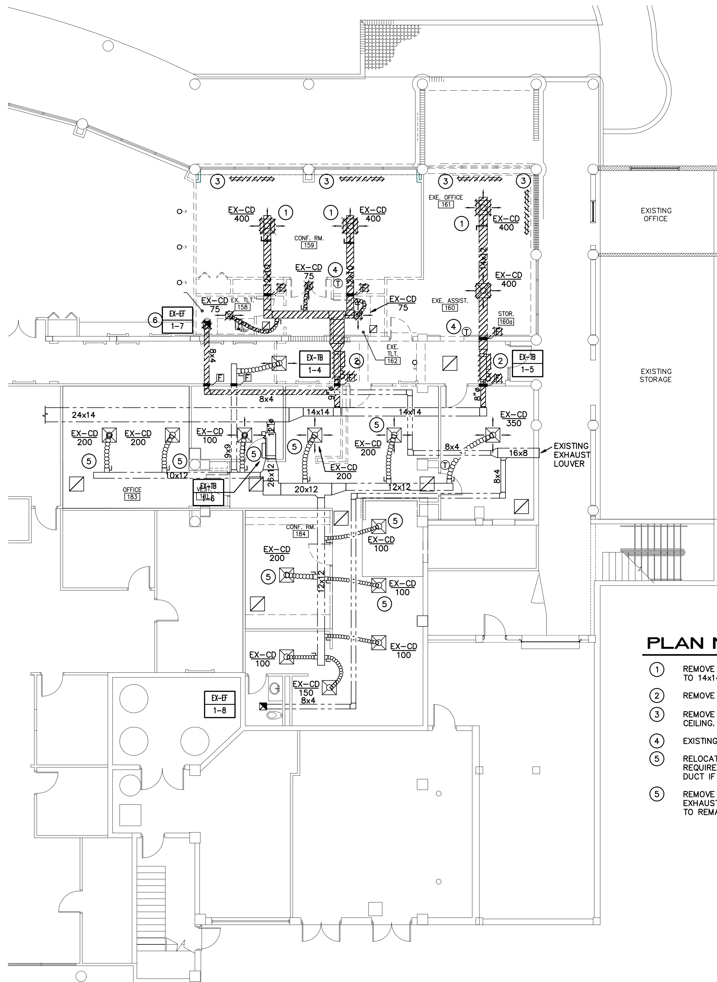
1 ADMINISTRATION MECHANICAL HVAC PLAN - DEMOLITION SCALE: 1/8" = 1'-0"
