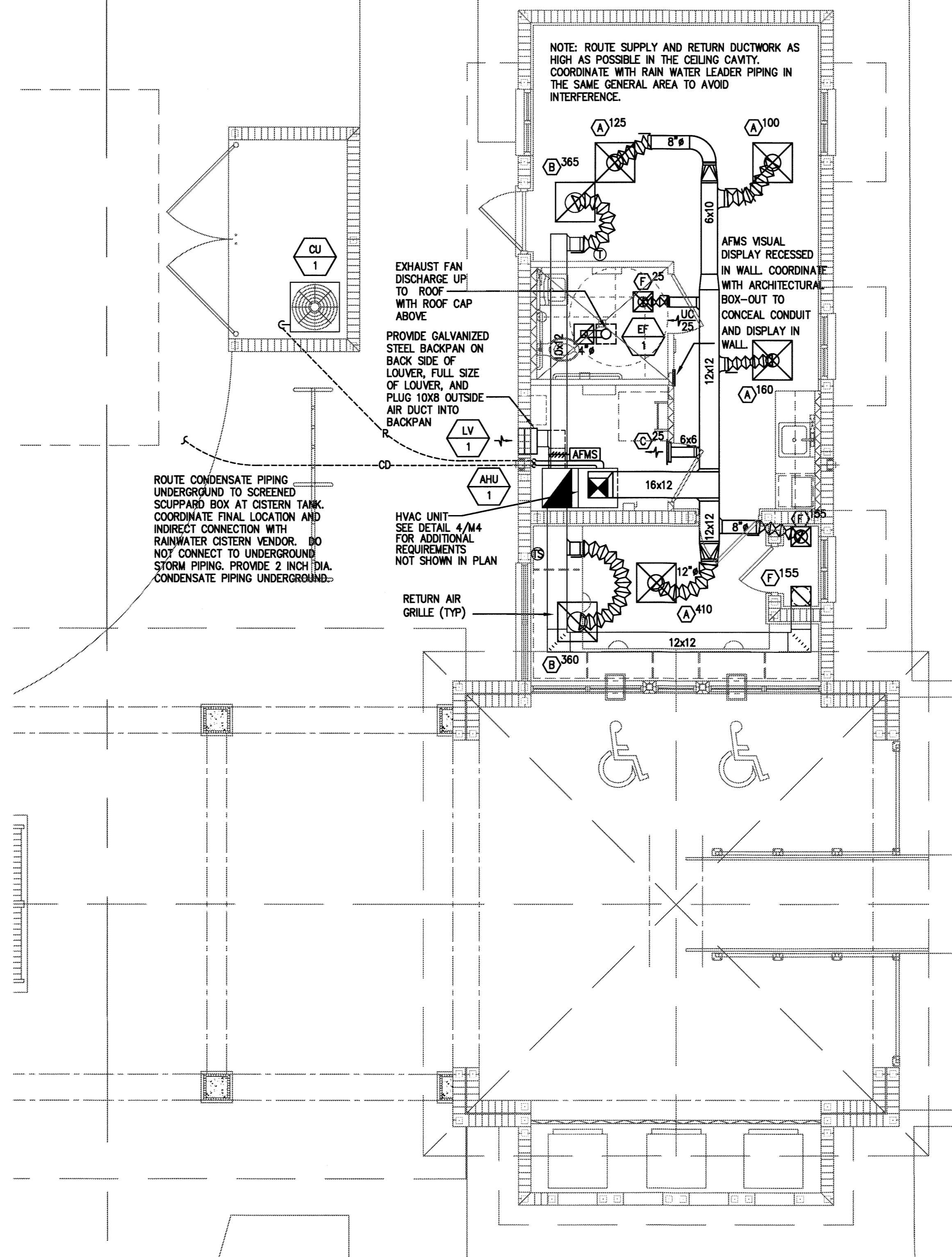
TICKET BUILDING FLOOR PLAN - MECHANICAL 1/4" = 1'-0"
