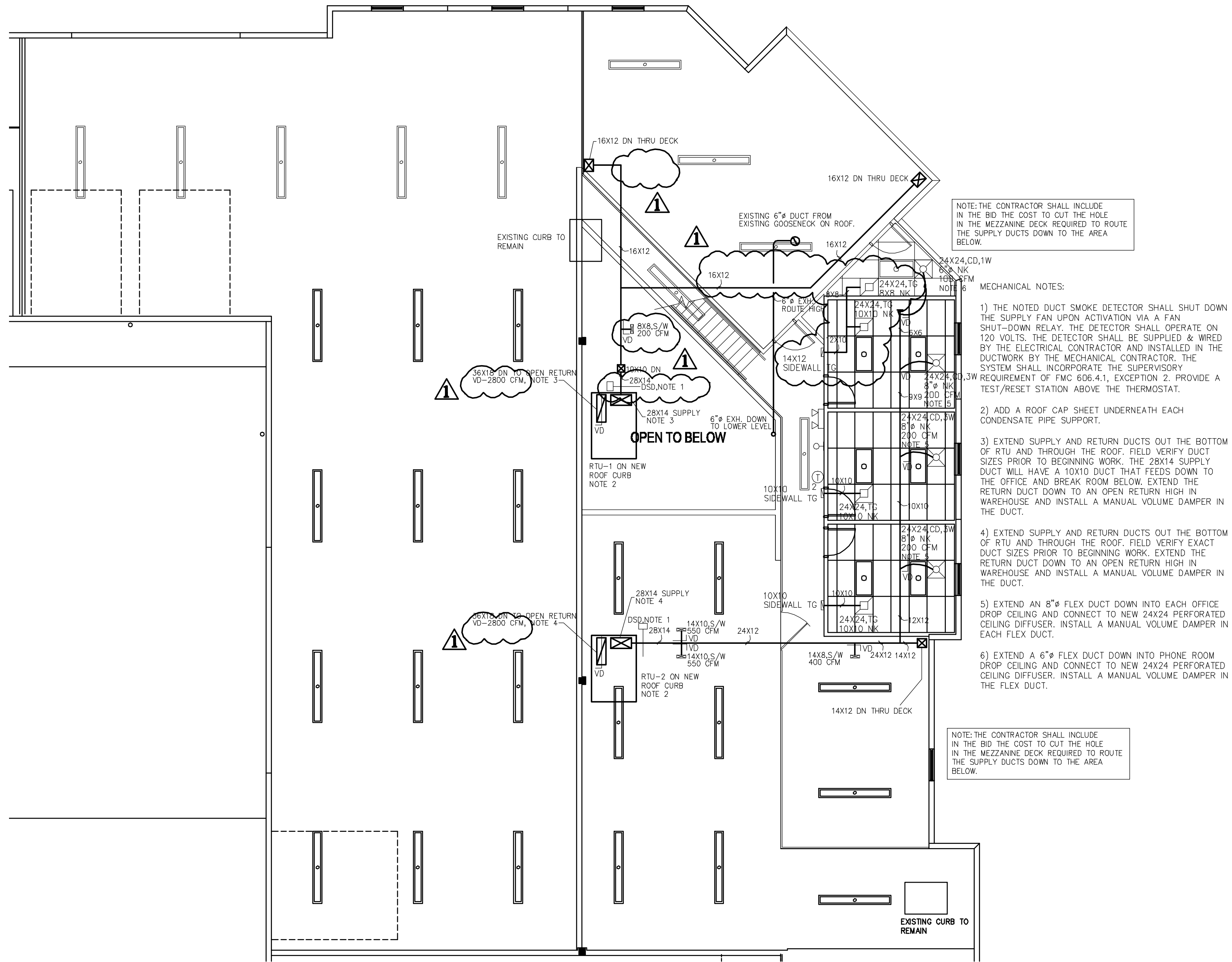
UPPER HVAC PLAN
